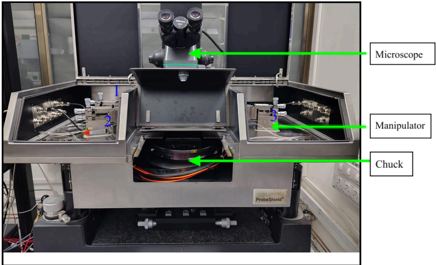
Probe station
